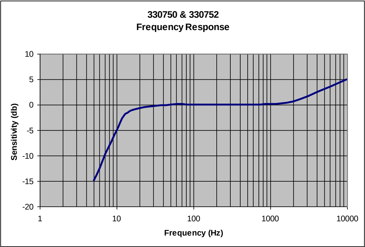
Figure 3: Velocity Amplitude
