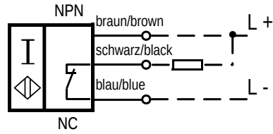
3RG4013-0GA00-PF:
