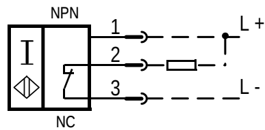
3RG4013-3GA00-PF:
