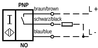
3RG4022-0AG30-PF:
