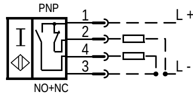
3RG4023-3CD00-PF / 3RG4023-2CD00-PF:
