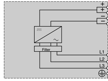
ABL7UES / UPS●●●●●
