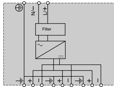
ABL7UES / UPS●●●●●
