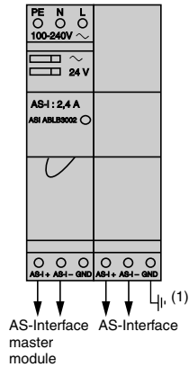
ASIABLB300●
