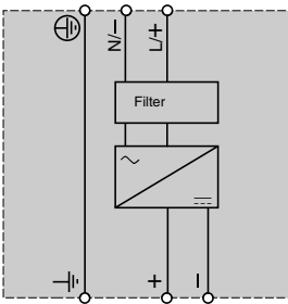
ABL7CEM24●●●
