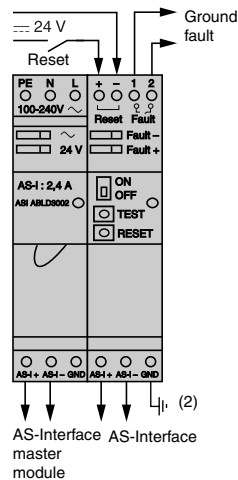
ASIABLD300●
