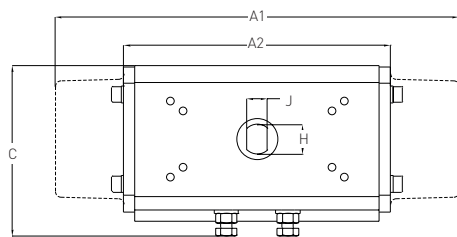
Top view model 002 – 020
