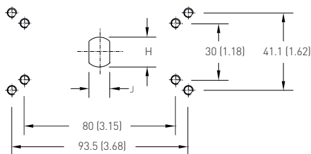
Top mounting drilling sizes 002 - 020
