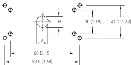
Top mounting drilling sizes 032 - 052
