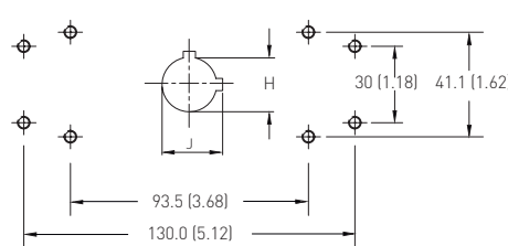
Top mounting drilling sizes 084 - 240
