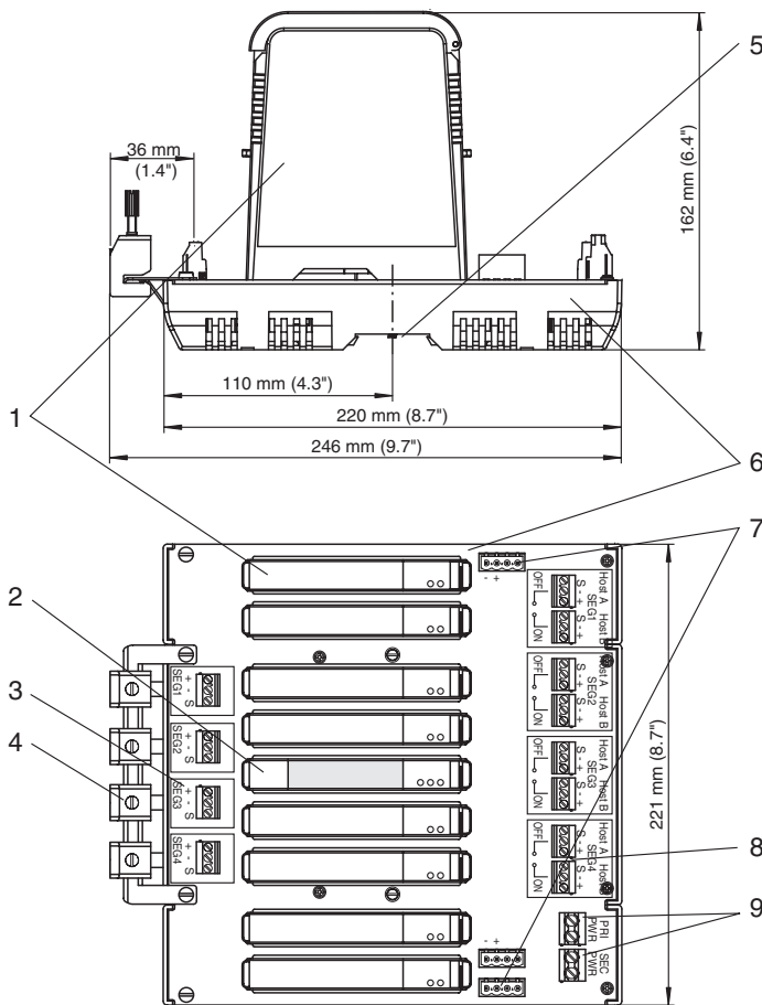
Dimensions complete redundant system*
