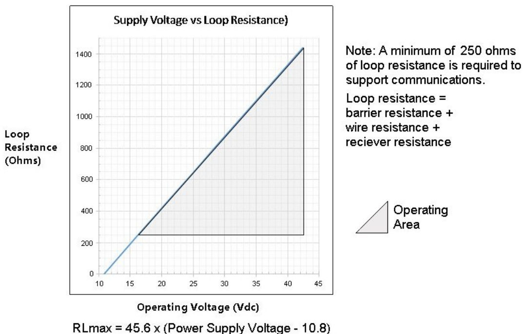
Figure 2 - Supply voltage and loop resistance chart &amp; calculations
