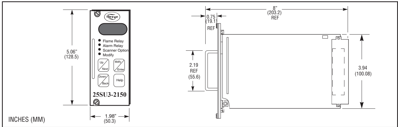
FIGURE 1. 25SU3 -2150 DIMENSIONS
