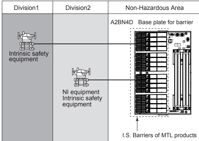
Figure Connection of A2BN4D for FM and CSA (1)
