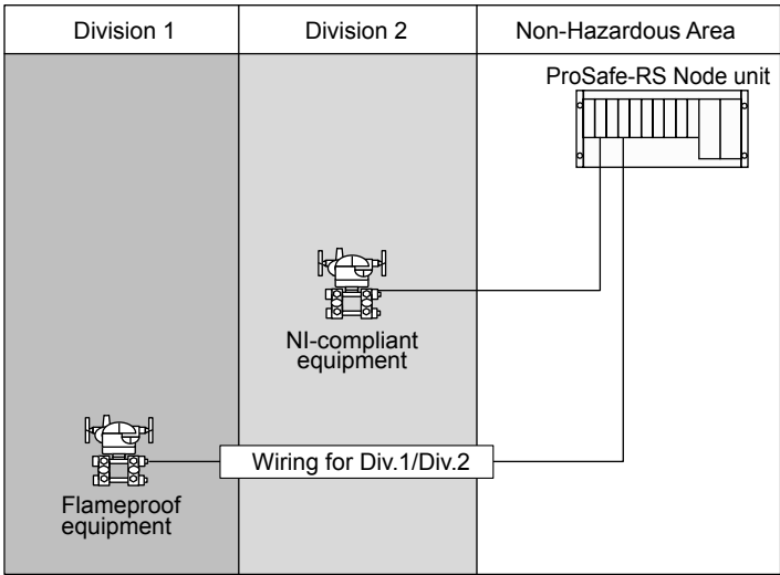
Figure NI (Flameproof Wiring)
