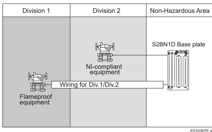
Figure Connection of S2BN1D for FM and CSA (1)
