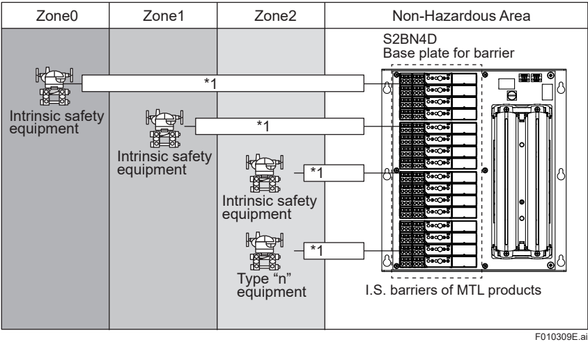
Figure Connection of S2BN4D for ATEX and IECEx (1)
