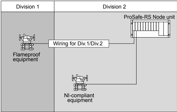
Figure NI (Installation in Division 2)
