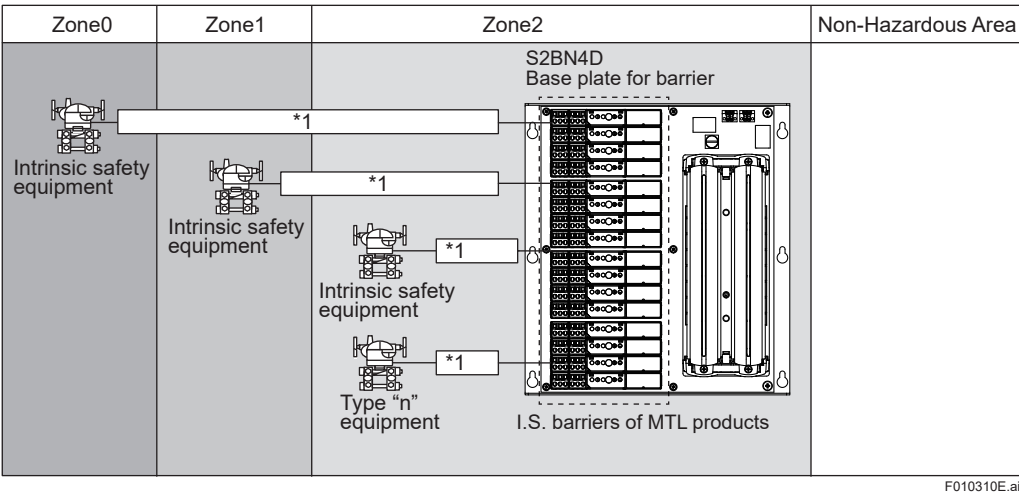
Figure Connection of S2BN4D for ATEX and IECEx (2)
