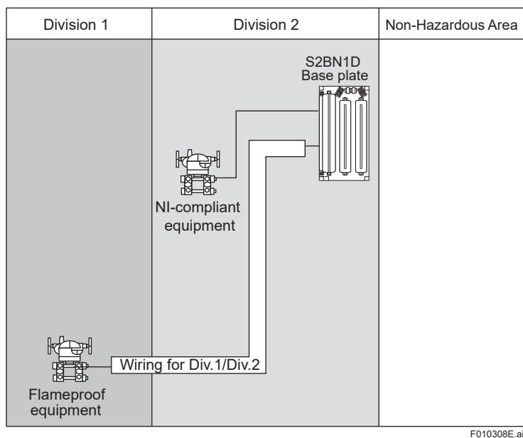
Figure Connection of S2BN1D for FM and CSA (2)
