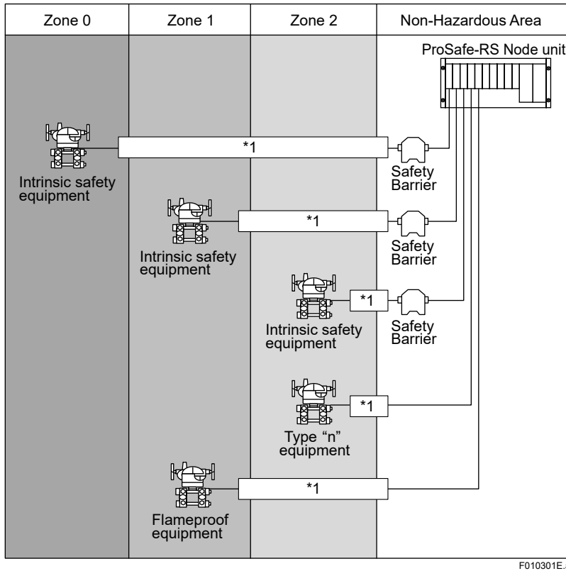
Figure Type “n”
