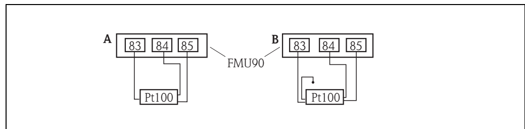
A Pt100 with 3-wire connection B Pt100 with 4-wire connection (one connector remains unused)
