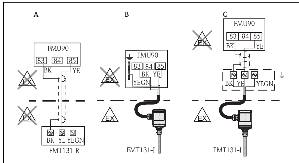
A Non-Ex area (FMT131-R) BK black B Ex area (FMT131-j) with grounding in the FMU90 YE yellow C Ex area (FMT131-j) with grounding at a terminal box YEGN yellow-green
