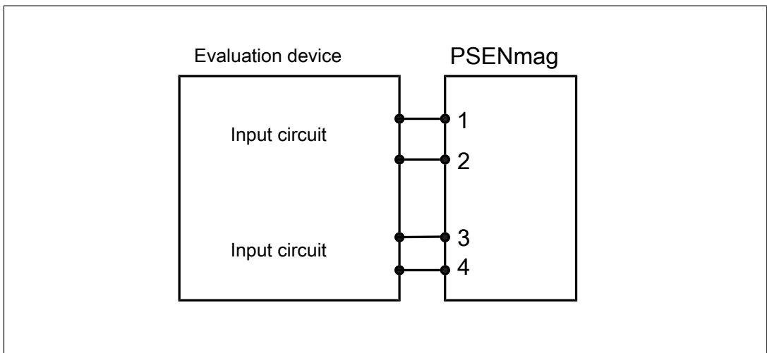
Fig.: Dual-channel connection PSEN ma1.1p-10 to the input circuits of an evaluation device
