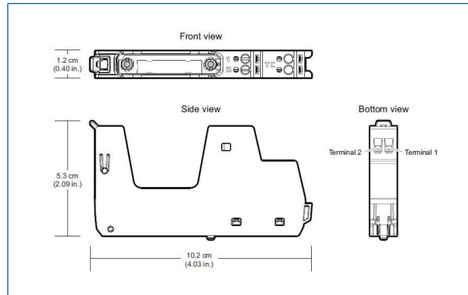
CHARM Thermocouple / mV Terminal Block.
