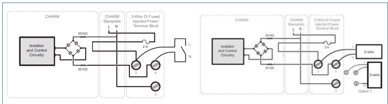
Simplified Circuit and Connection Diagrams for DI 230V AC Isolated CHARM with 3-wire DI Fused-Injected-Power Terminal Block.
