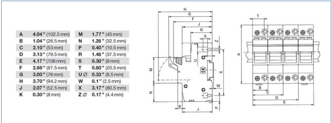
Outside Dimensions of the Fuse Holder.
