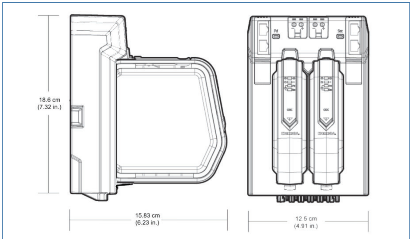
CHARM I/O Card and Carrier.
