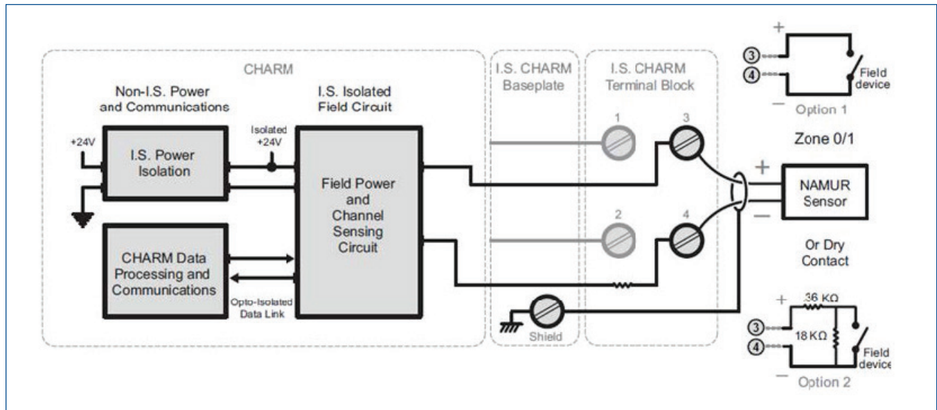
Simplified Circuit and Connection Diagram for IS DI NAMUR CHARM.
