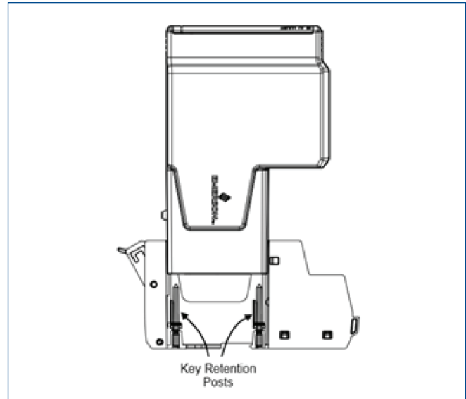
IS CHARM Terminal Block.
