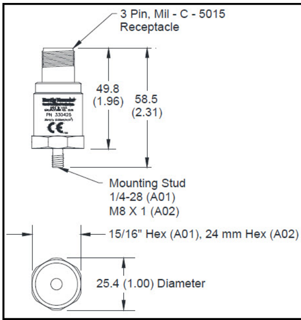
330400/330425 Accelerometer Sensor
