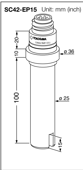
Figure 6 Insertion type
