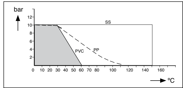
Figure 18 Pressure/temperature class
